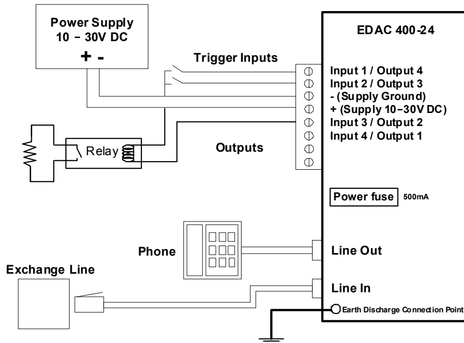
Figure 1: Typical EDAC 400-24 Installation
